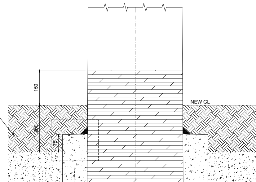
WATER PROOFING Scale 1:10
