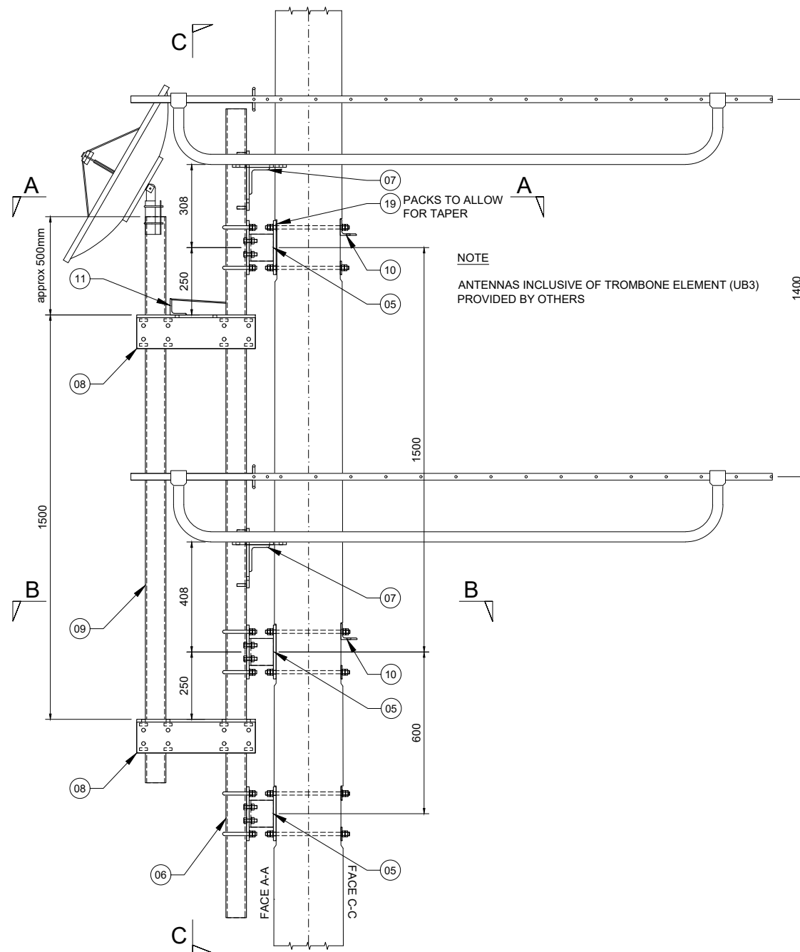
DETAIL G - ANTENNA MOUNTS Scale 1:20
