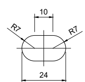
SLOTTED HOLE DETAIL Scale 1:2
