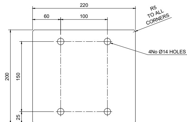
TPB-B-1 - 10mm THICK Scale 1:5
