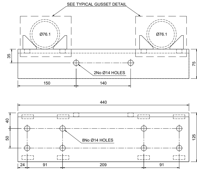
TPA-M - UA125x75x10 Scale 1:5
