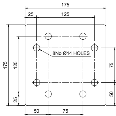
TPA-BR-4 - 10mm THICK Scale 1:5
