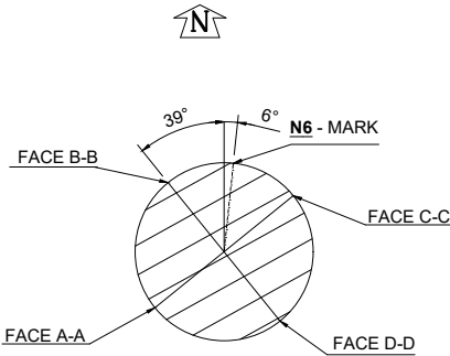
POLE ORIENTATION Scale 1:20
