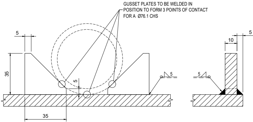
TYPICAL GUSSET PLATE DETAIL Scale 1:2
