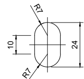
SLOTTED HOLE DETAIL Scale 1:2
