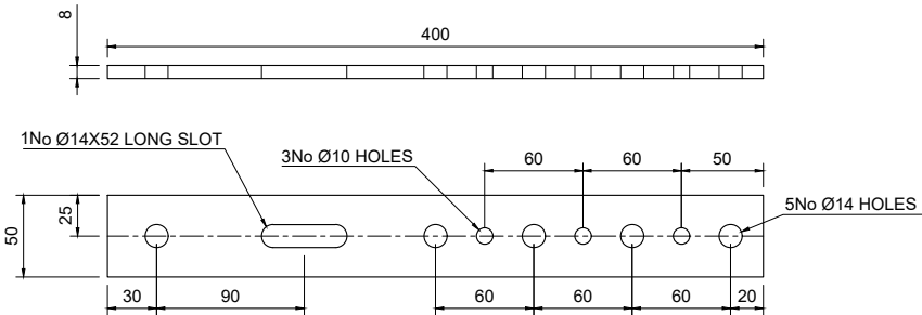
TPA-PD - 8mm THICK Scale 1:5
