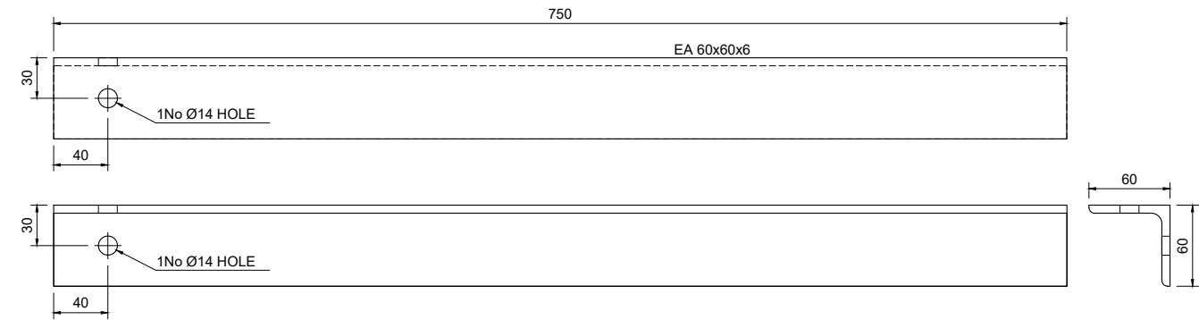
TPA-BR-1 - EA60x60x6 Scale 1:5
