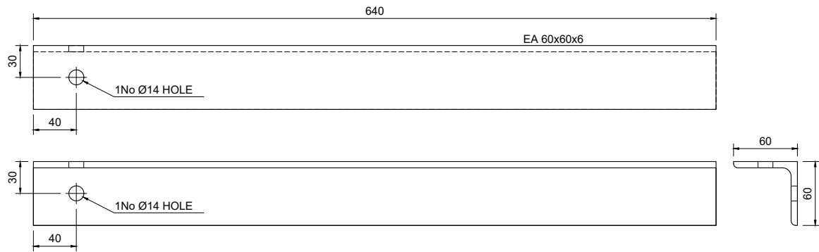
TPA-BR-2 - EA60x60x6 Scale 1:5
