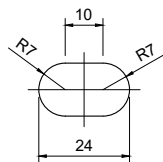
SLOTTED HOLE DETAIL Scale 1:2
