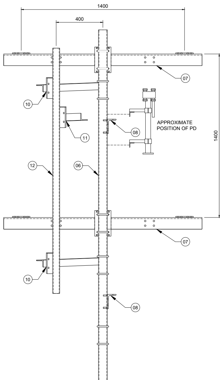
SECTION C-C Scale 1:20
