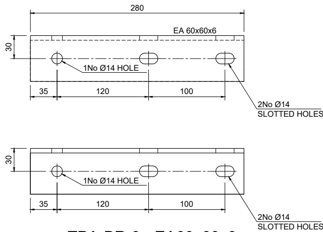
TPA-BR-3 - EA60x60x6 Scale 1:5
